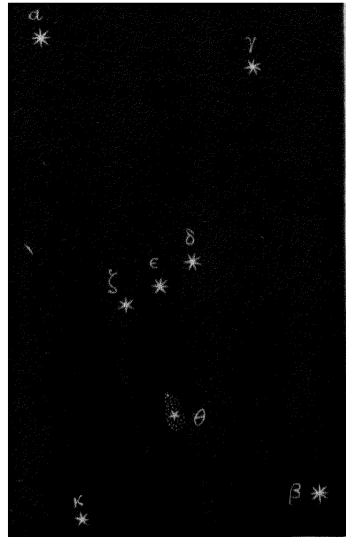
FIG. 10. ORION.
