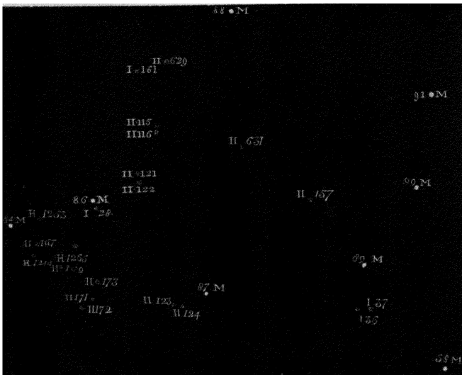
FIG. 21. GROUP OF NEBULÆ IN VIRG.
