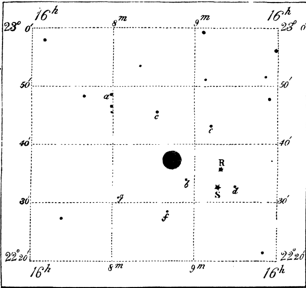
FIG. 33. VARIABLE STARS NEAR 80 M. SCORPII. (EPOCH, 1860).
